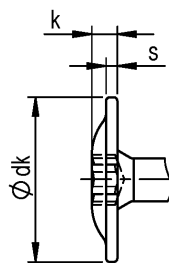
Tellerkopf
