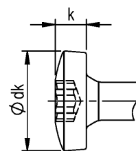
Pan Head / Linsen Kopf
