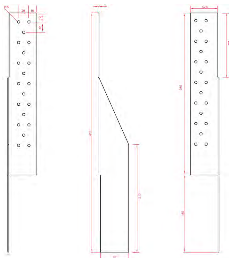
Figure B.20 Dimensions of vertical flange BPR465 S250 for two-piece hold-downs
