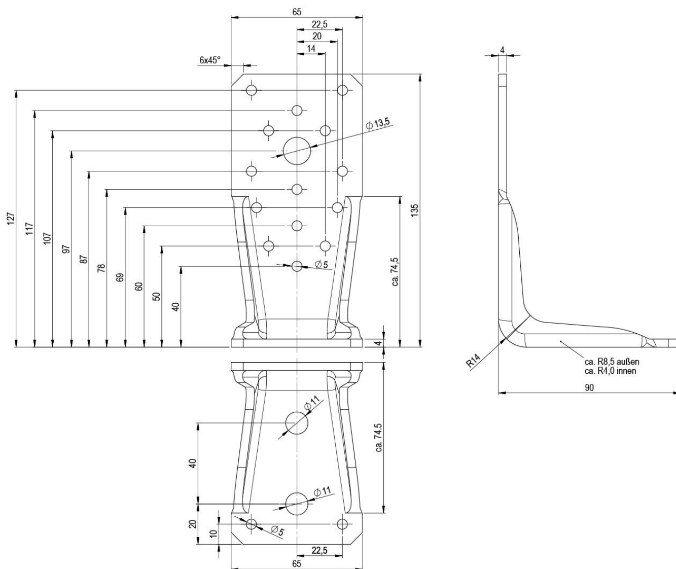
Figure B.36 Dimensions of type KR RL 135x65x4,0_Ø11
