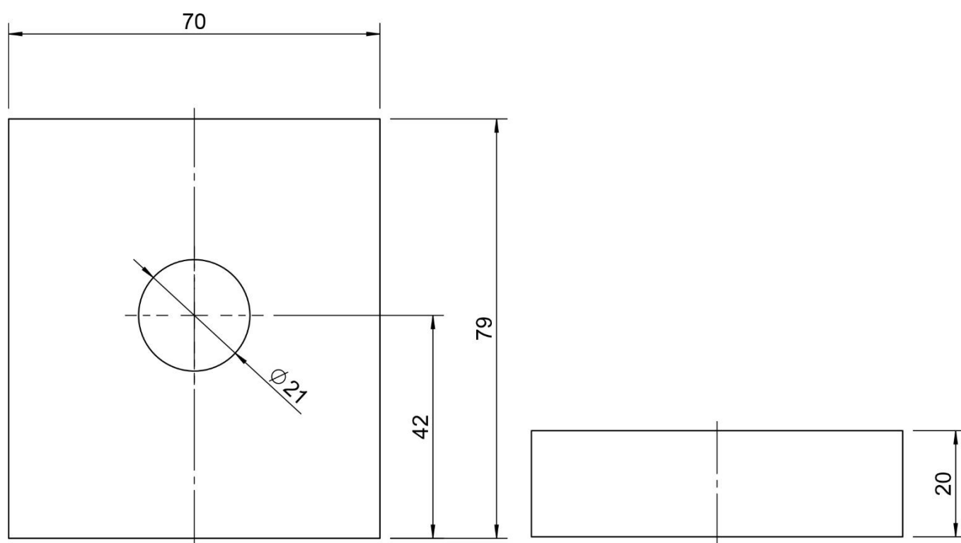
Figure B.10 Dimensions of base plates type R Lx79x70x20 \varnothing 21
