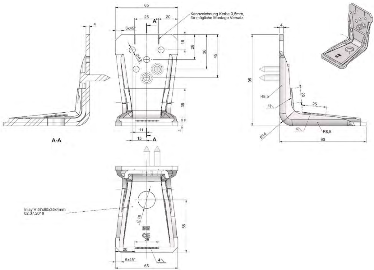
Figure B.13 Dimensions of two-piece hold-down type KR 95x90x65x4,0
