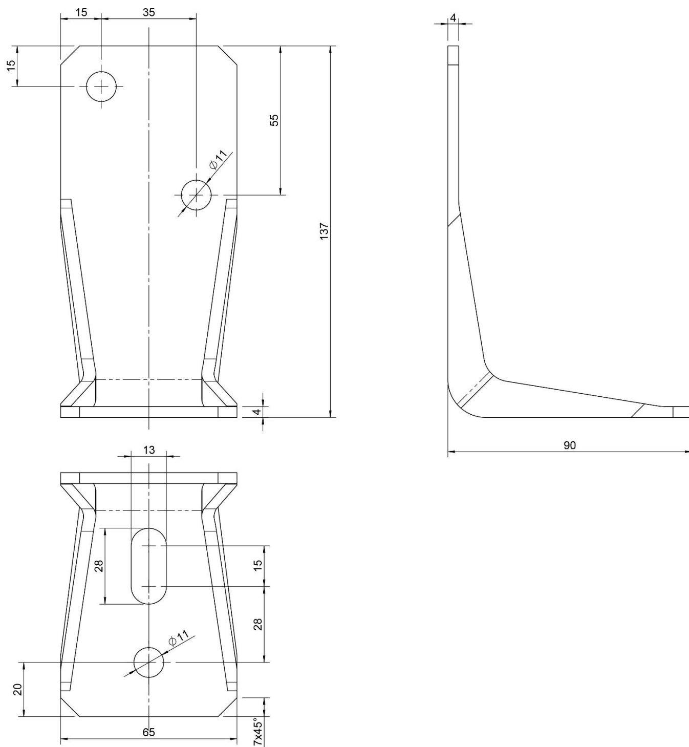
Figure B.30 Dimensions of type KR LL 137x65x4,0
